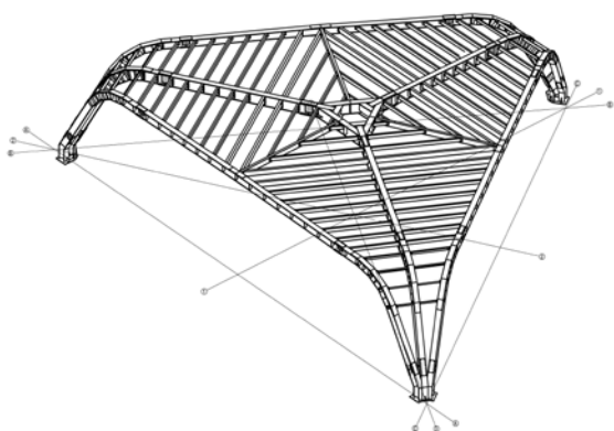
ISOMETRIC SCALE 1:100
