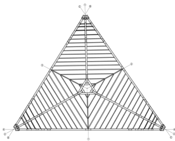
STRUCTURE PLAN SCALE 1:100
